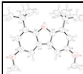
Fig. 1. The structure of the title compound with displacement ellipsoids drawn at 50% probability level.
