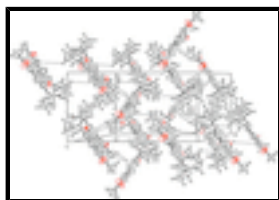
Fig. 2. A packing diagram of the title compound. Dashed lines represent C—H... \pi interactions.
